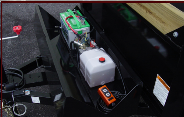
Pump & Battery Box
